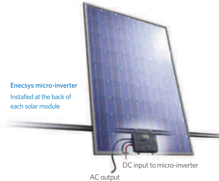
Enecsys micro-inverter
